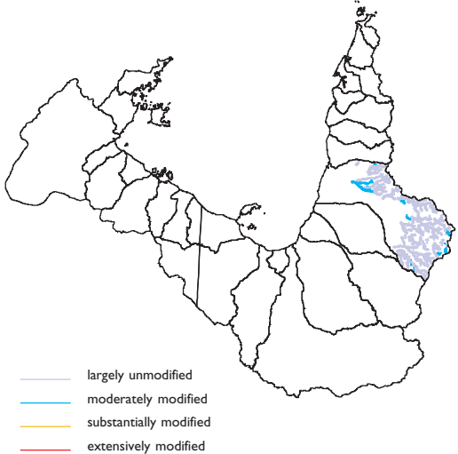
RIVER CONDITION (environment index by reach) ESTUARY CONDITION (condition for each
