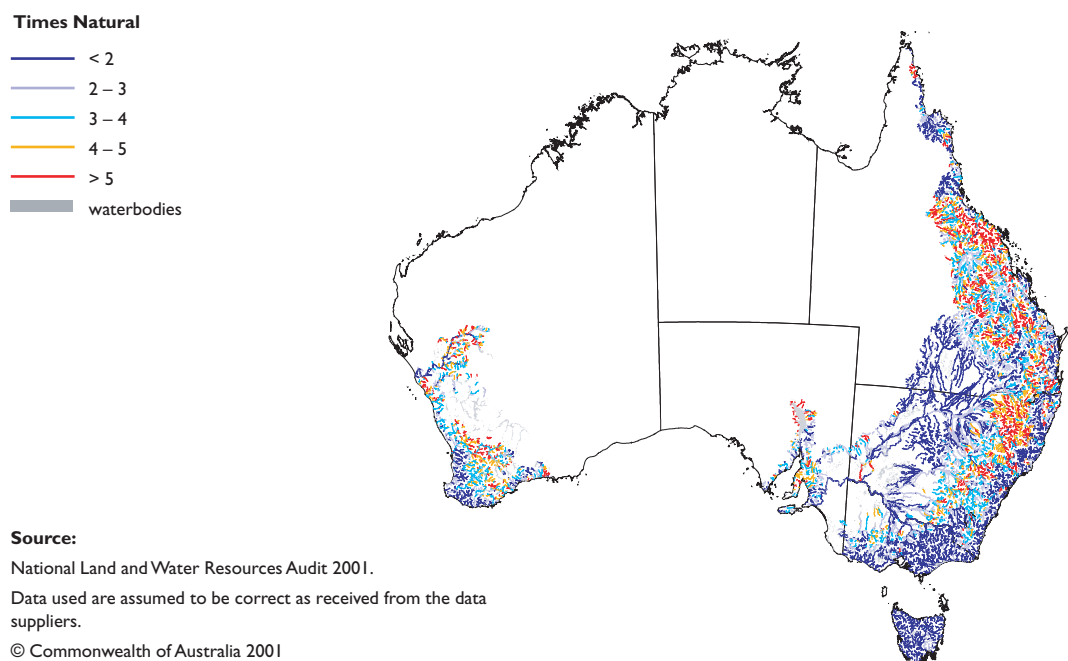
Figure A13 Relative increase in average annual total nitrogen load by river network (NLWRA 2001b).
