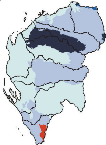
LANDSCAPE STRESS (composite index by subregion)
