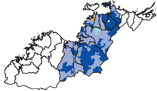
CATCHMENT CONDITION (composite score by 500 km 2 subcatchment)
