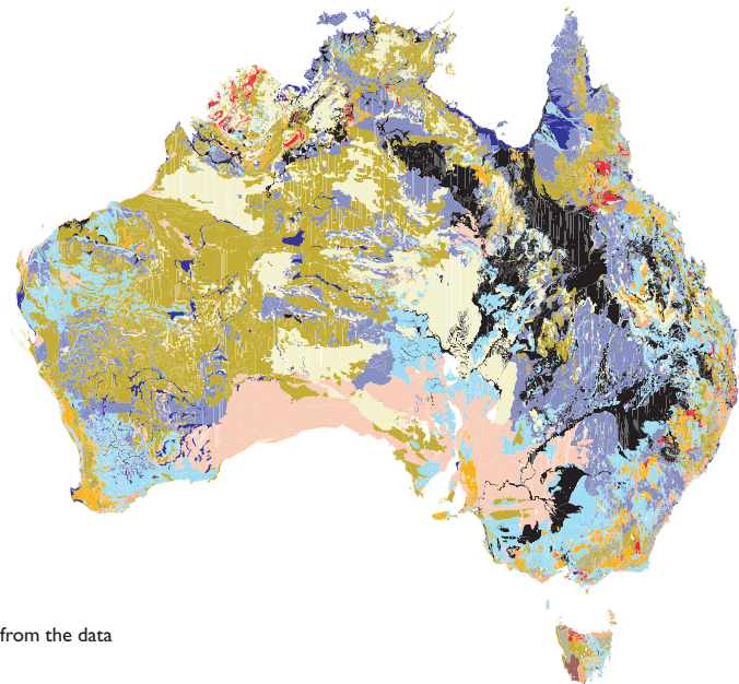
Figure A4 Australia's soil orders according to the Australian Soil Classification (NLVRA 2001b).
