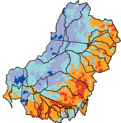
CATCHMENT CONDITION (composite score by 500 km 2 subcatchment)
