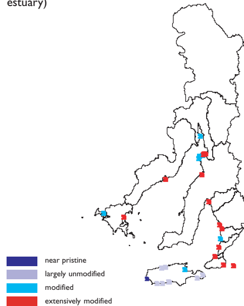
ESTUARY CONDITION (condition for each estuary)
