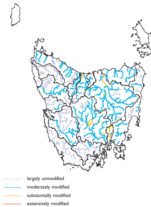
RIVER CONDITION (environment index by reach)
