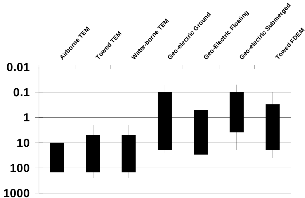
Figure 3 Ranges of detectable depths of various EC imaging devices (in metres). Note that airborne FDEM (not shown) has a range similar to but shallower than airborne TEM.
