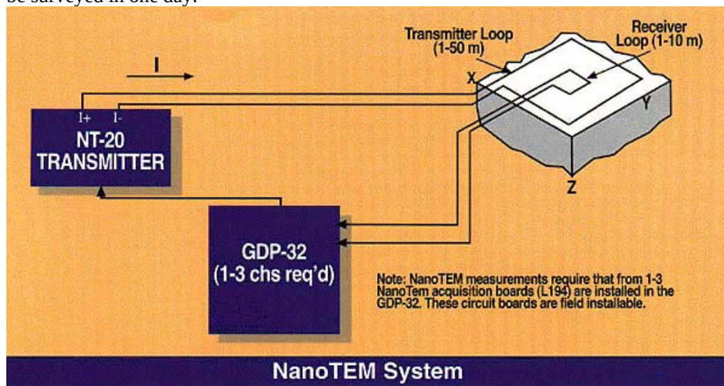
Figure 43 A schematic of the NanoTEM system in operation.
