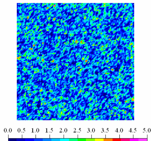
Figure 4.3 Stochastic distribution of hydraulic conductivity (1 cm/day, coefficient of variance \sim 30\% ) in a 100 cm x 100 cm domain
