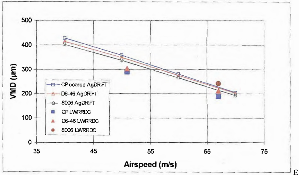
Figure 9. The effect of airspeed on droplet size
