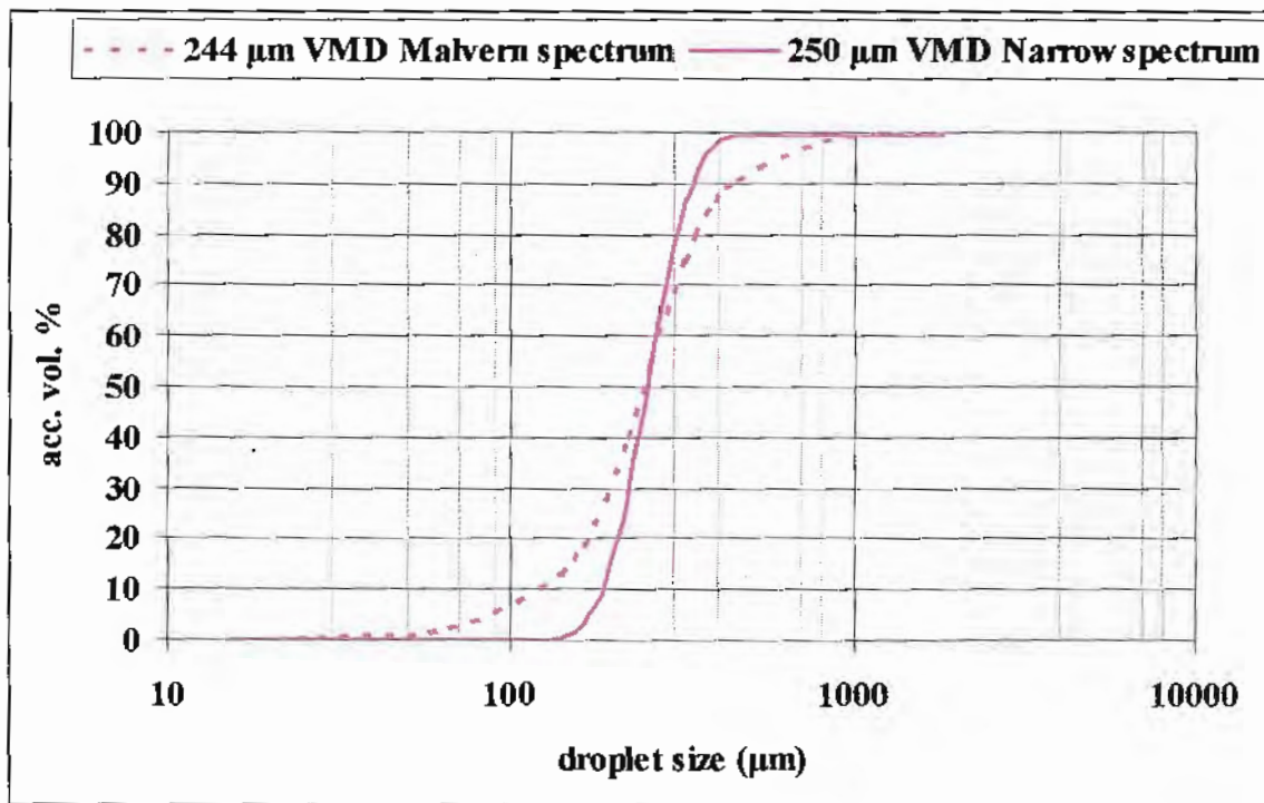
Figure 8. Computer generated 250 \mu\text{m} VMD narrow spectrum compared to 244 \mu\text{m} VMD Malvern data
