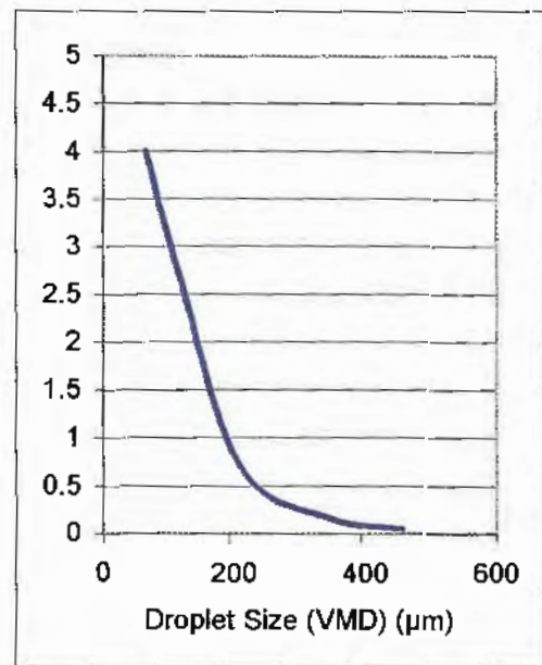
Figure 4. Summary of application parameters on aircraft spray drift. Drift expressed as percentage of applied rate deposited 500 metres downwind of field. (all apart from turbulence intensity were carried out using AgDRIFT™).
