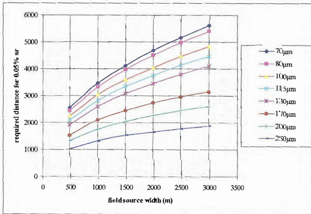
Figure 6. Effect of field source width on spray drift buffer distance required to reach 0.05% field applied rate
