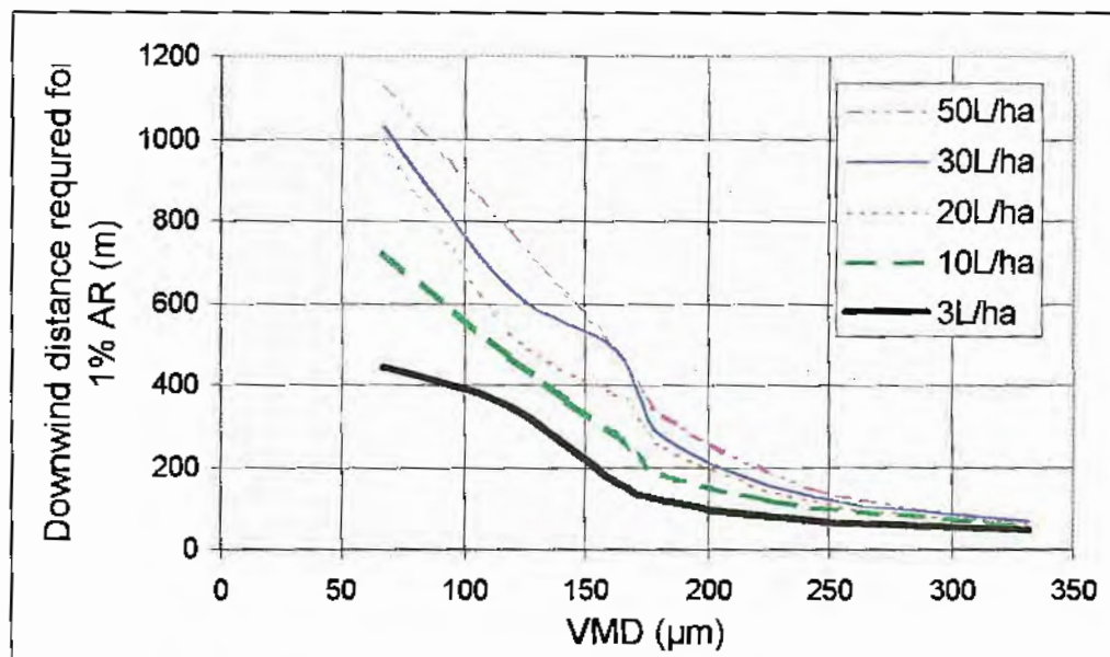
Figure 10. Effect of droplet size (VMD) on downwind buffer distances required for deposition to fall to 1% of applied rate (AR) for various total application rates (constant product rate of 2.1 L/ha)
