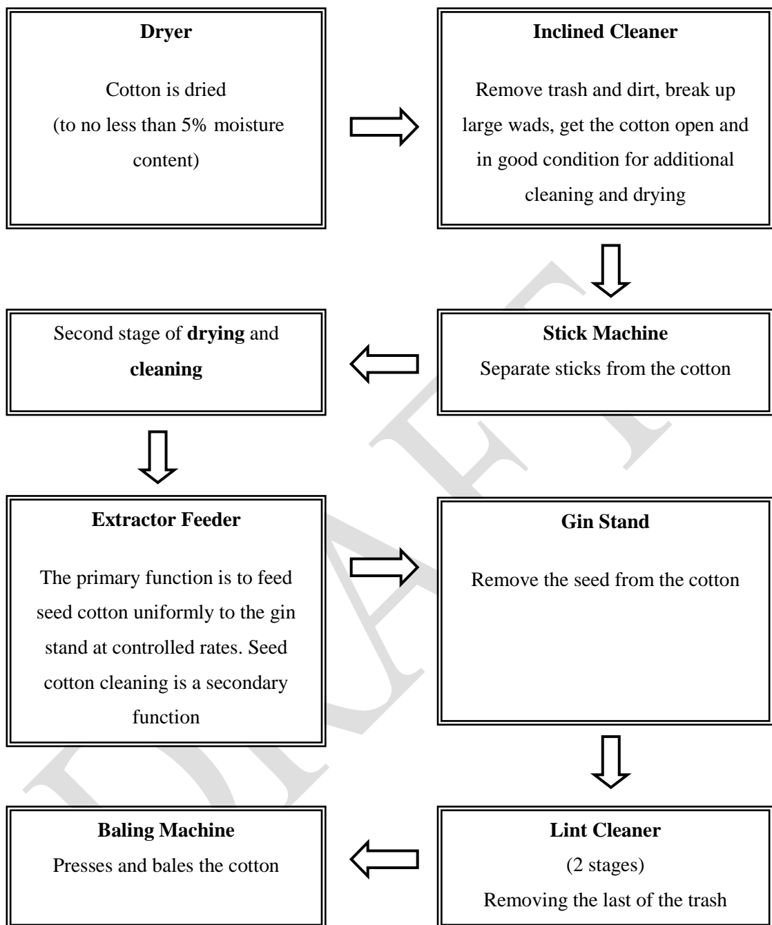
Figure 3.1: Sequence of the ginning process
