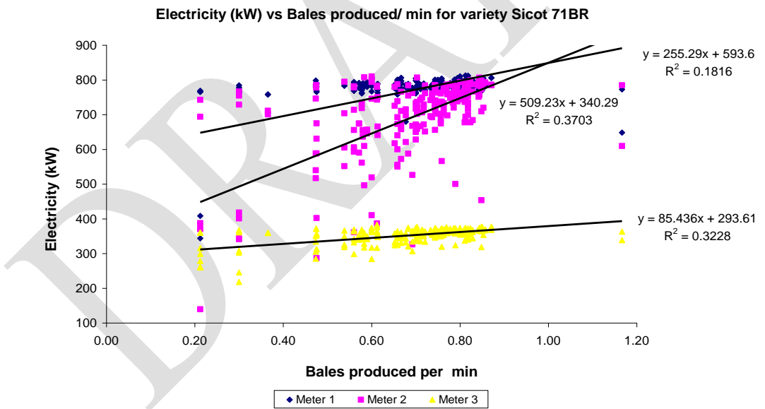
Figure A 7.6: Relationship between electricity (kW) with bales produced for Sicot 71BR
