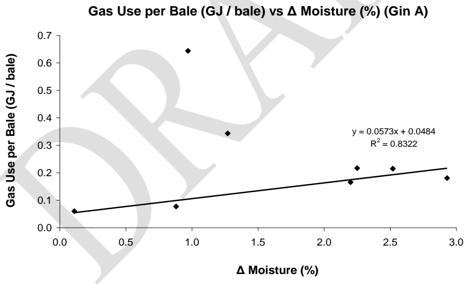
Figure 5.4: Relationship between gas consumption (GJ)/ bale with Δ moisture (Gin A) Note: The two largest results, with respect to the y-axis, were found to be outliers and were removed from the regression.
