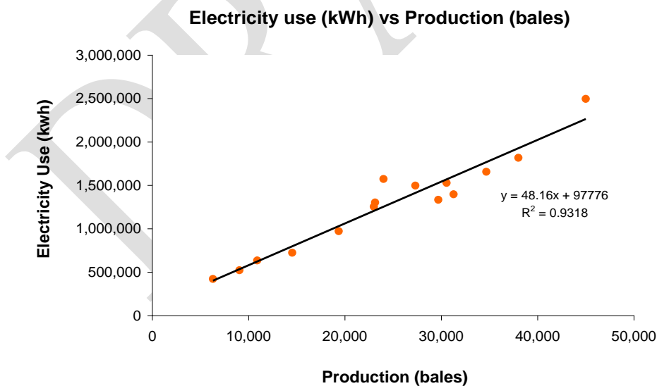
Figure 4.3: Relationship between electricity consumption (kWh) and production (bales)
