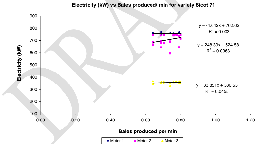
Figure A 7.4: Relationship between electricity (kW) with bales produced for Sicot 71
