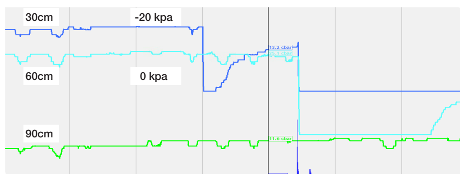
Figure 1 Typical graphed gm sensor data with a moveable cursor displaying readings at 30, 60 and 90 cm of soil depth in centi-bars of soil tension. 1 centi-bar = 1 kilopascal. Figures do not display negative notation. Rainfall displays in vertical blue bars, irrigation in vertical green bars. Adcon Telemetry.
