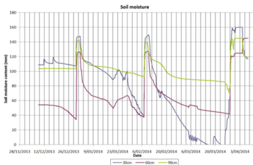
Sample output for calibrated MP406 soil moisture sensors installed at three depths:
