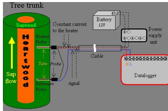
Figure 2.11: Schematic of Granier's thermal dissipation sap flow sensors (Source: www.plantsensors.com/ )
