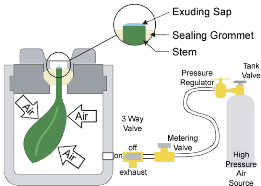
Figure 2.2: Operation of a pressure chamber to measure plant water status
