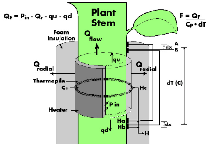
Figure 2.9: Principal of operation for the Dynagage sap flow sensor
