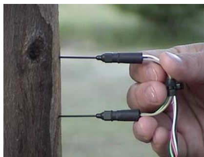
Figure 2.10: Thermal dissipation probe
