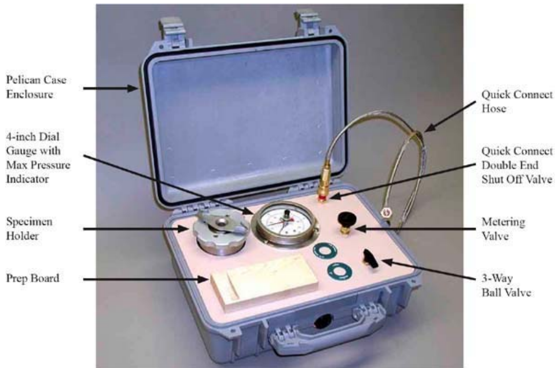
Figure 2.1: Portable pressure chamber and console (Source: http://www.ictinternational.com.au/PortablePWSC.htm )
