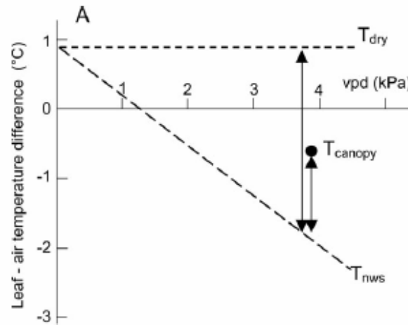
Figure 3.7: Illustration of CWSI noting the upper ( T_{dry} ) and lower ( T_{nws} ) baseline temperature values across a range of VPD (represented by dashed lines) and a normalised leaf temperature value ( T_{canopy} ) found between this range.
