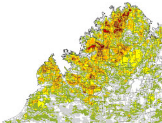
Figure 31. Remotely sensed image showing fire frequency in the Kimberley.
