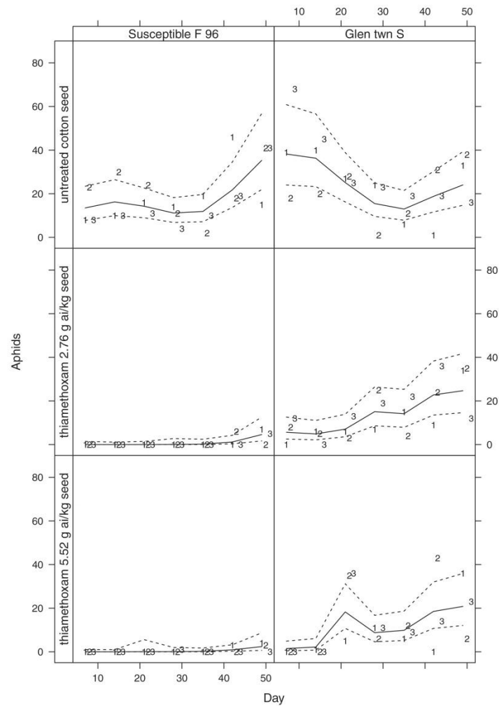
Fig. 1. Fitted trend for the thiamethoxam analysis, for each strain by treatment combination (thiamethoxam at 5.52 g a.i./kg seed, Cruiser Extreme ® Insecticide Seed Treatment; thiamethoxam at 2.76 g a.i./kg seed, Cruiser ® Insecticide Seed Treatment; untreated cotton seed, variety Sicot 71). The solid line represents the fitted trend, with dotted lines representing the 95% confidence interval. The raw data for each replicate is numbered 1 to 3 in each panel (with replicates 1 and 3 shifted slightly left and right, respectively, to avoid overlap).
