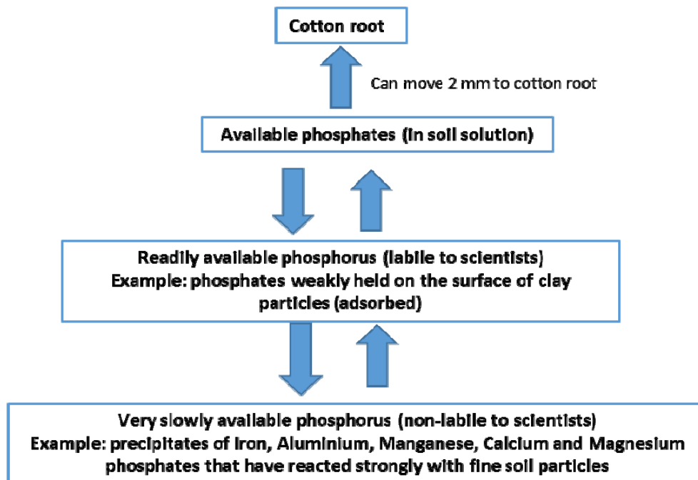
Figure 3. Simplified diagram of soil phosphorus pools (from Bailey, 2011).
