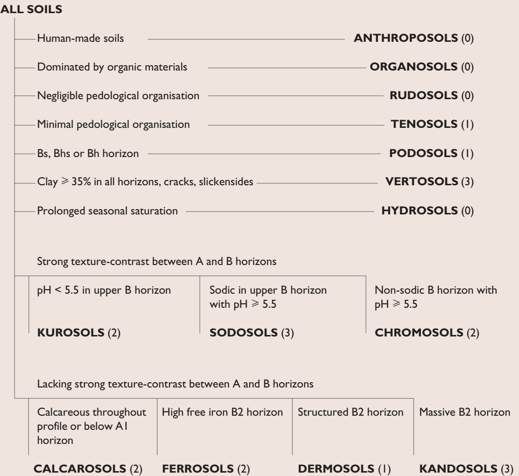
Figure 1. Schematic summary of the soil orders. Figures in parentheses refer to the number of soil profiles described in this chapter. The figure is not a key and readers are referred to Isbell (1996) if profile allocation is required.
