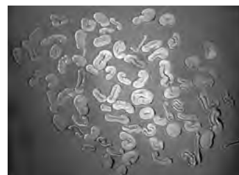
The cross section of a cotton yarn showing the packing and interaction of individual fibres. In this yarn cross-section seventy eight individual fibres are distinguishable. Changes in micronaire affect how many fibres make up the cross section of the yarn affecting its strength. (Photo: CSIRO)
