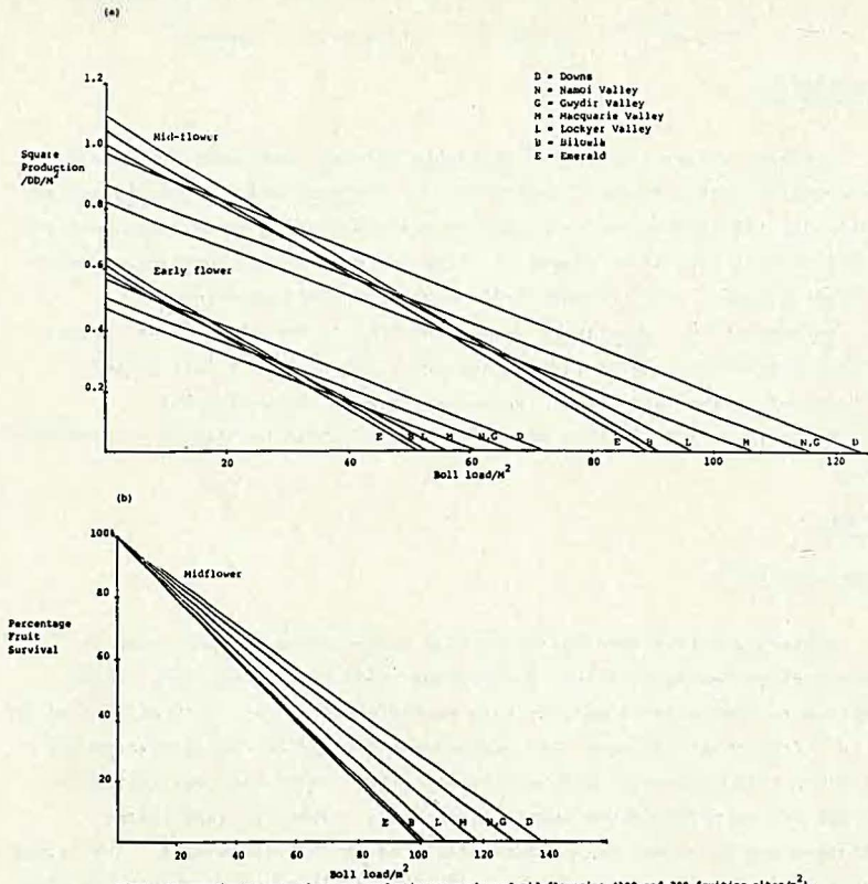
Fig 1. Changes in (a) rate of square production at early and mid-flowering (100 and 300 fruiting sites/m 2 ), (b) fruit survival at mid-flowering; with boll load for each region.
